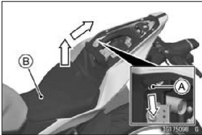
A. Seat Lock Cable B. Rider's Seat
