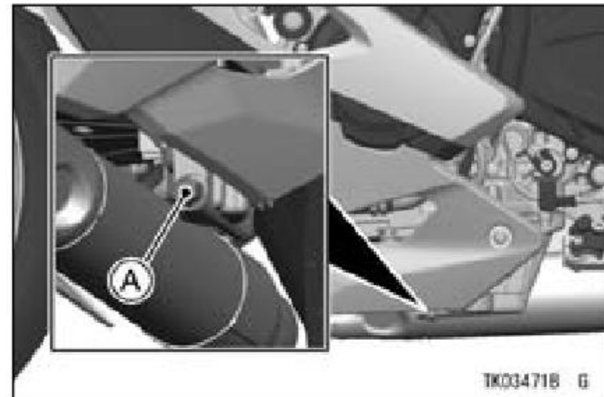
A. Engine Oil Drain Bolt
