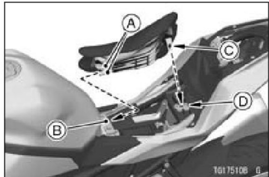
A. Hooks B. Fuel Tank Bracket C. Seat Latch D. Latch Hole
